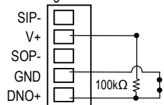
Sensor terminal block
